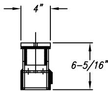
Low Lifting Adaptor
