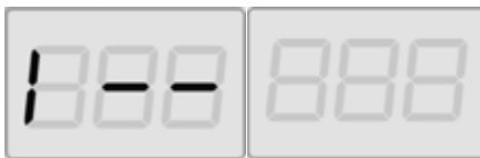
Fig. 24: Search for the balancing planes: the left display indicates to move the sensor back (move it to the left) to find the exact internal position of the balancing planes
