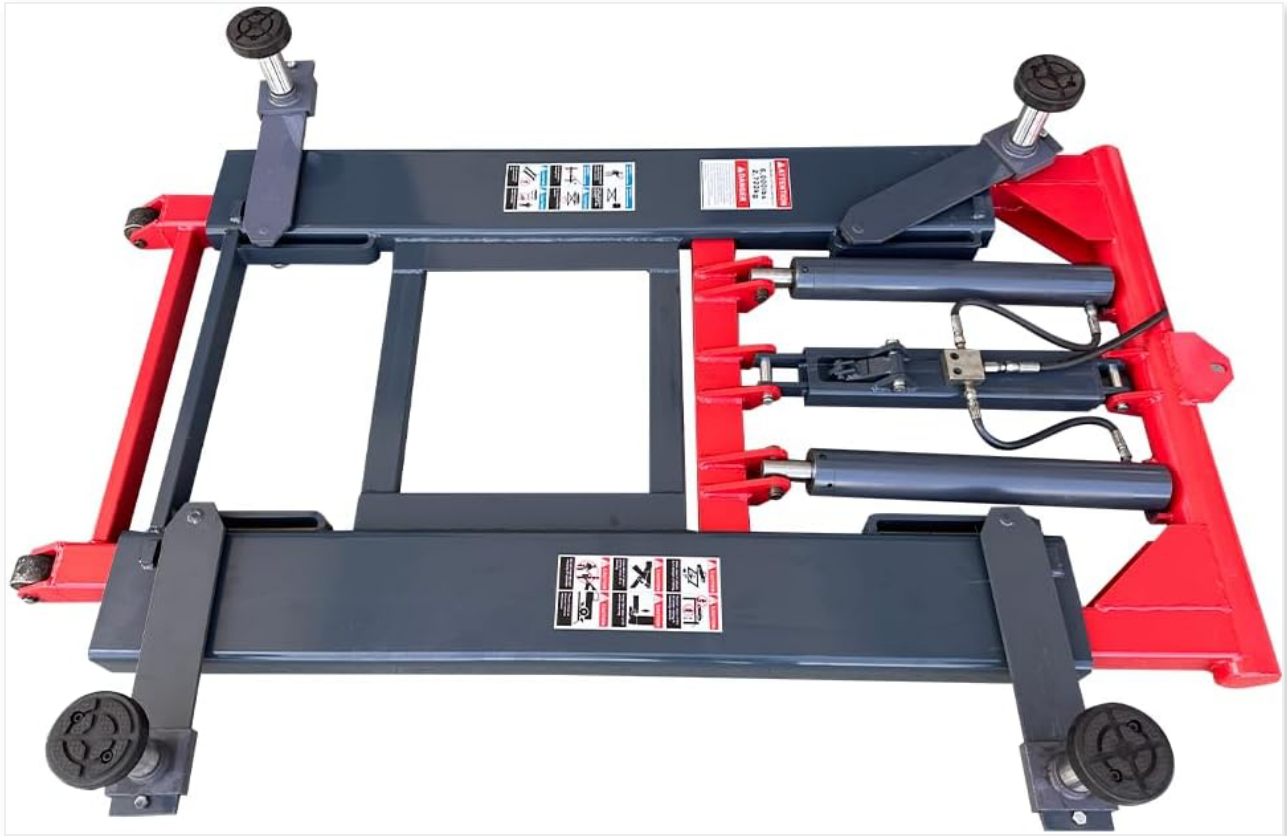
Figure 5.1: Top view of the KATOOL AK-X66 Scissor Lift, illustrating the hydraulic cylinders and structural frame in the lowered position.
