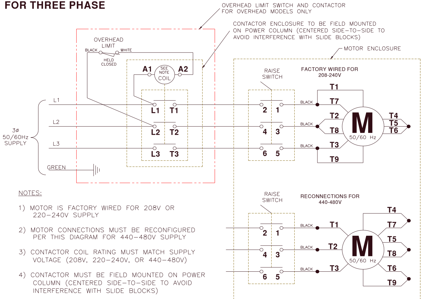
Fig 22 – Electrical Wiring Diagram
