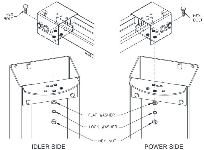
Fig 11 – Asymmetric Overhead Mounting
