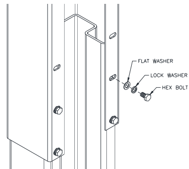
Fig 2 - Column Extension
