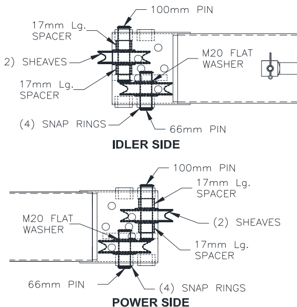
Fig 10 – Asymmetric Sheave Assembly
