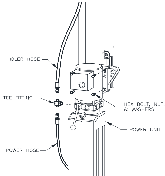
Fig 16 – Power Unit Assembly
