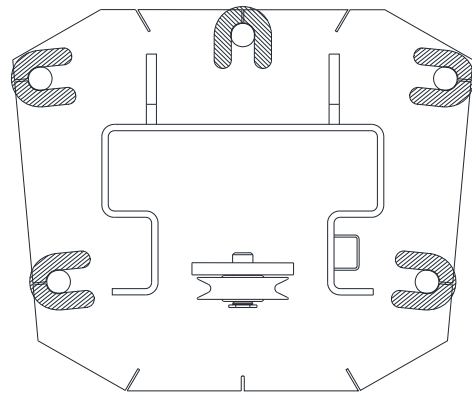
Fig 5 – Column Shimming
