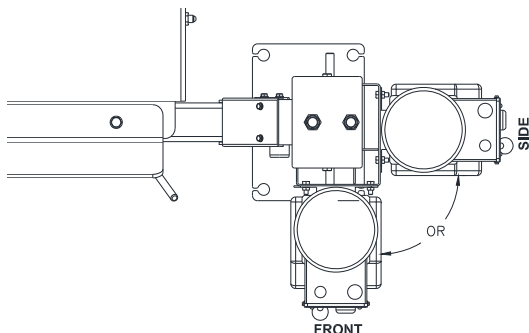
Fig 15 – Power Unit
