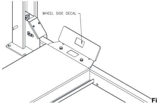
Fig 23 – Removable Wheel Stops
