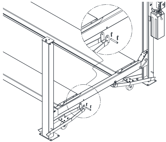
Fig 27 – Mobility Kit
