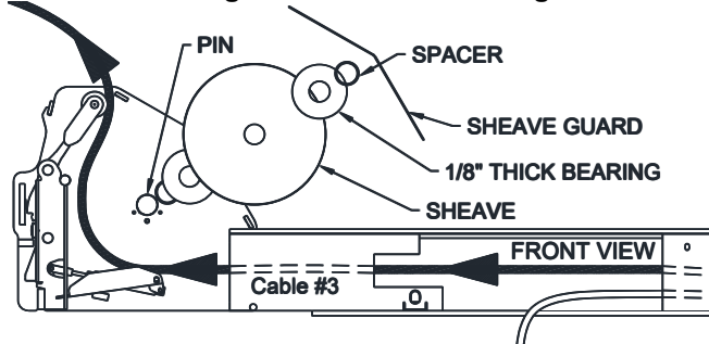
Fig 13 – Cable #3 Routing
