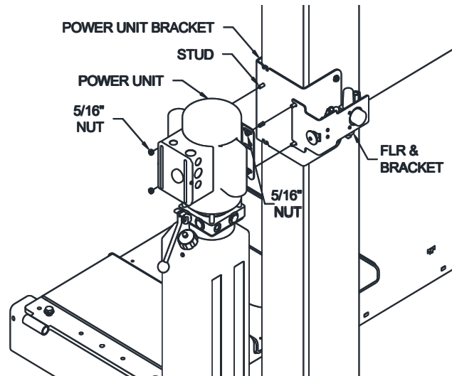
Fig 21b – Power Unit Bracket & Power Unit Mounting
